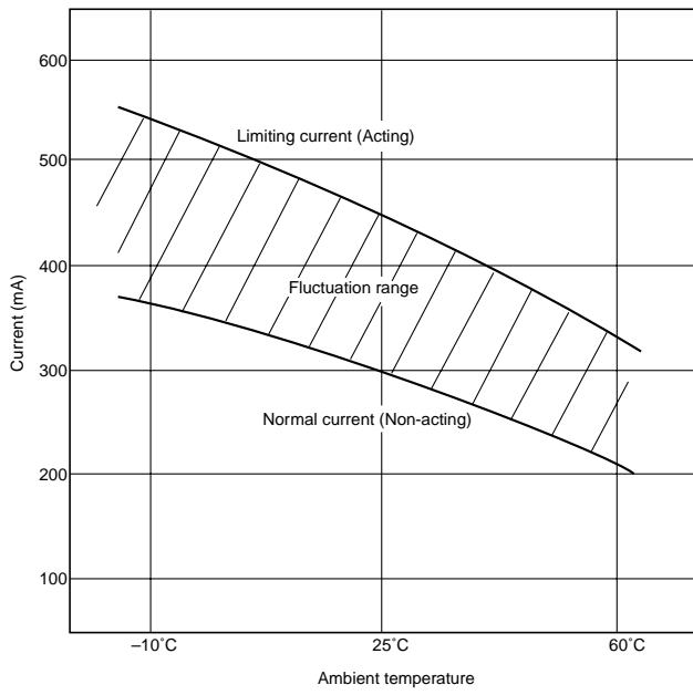
Fig. 10 Current Characteristics
