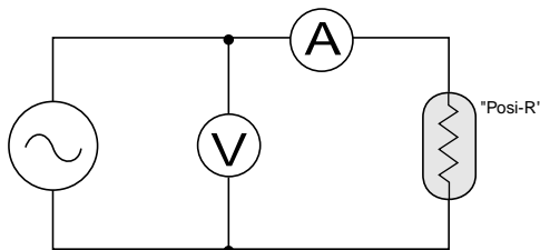
Fig. 3 Measuring Circuit
